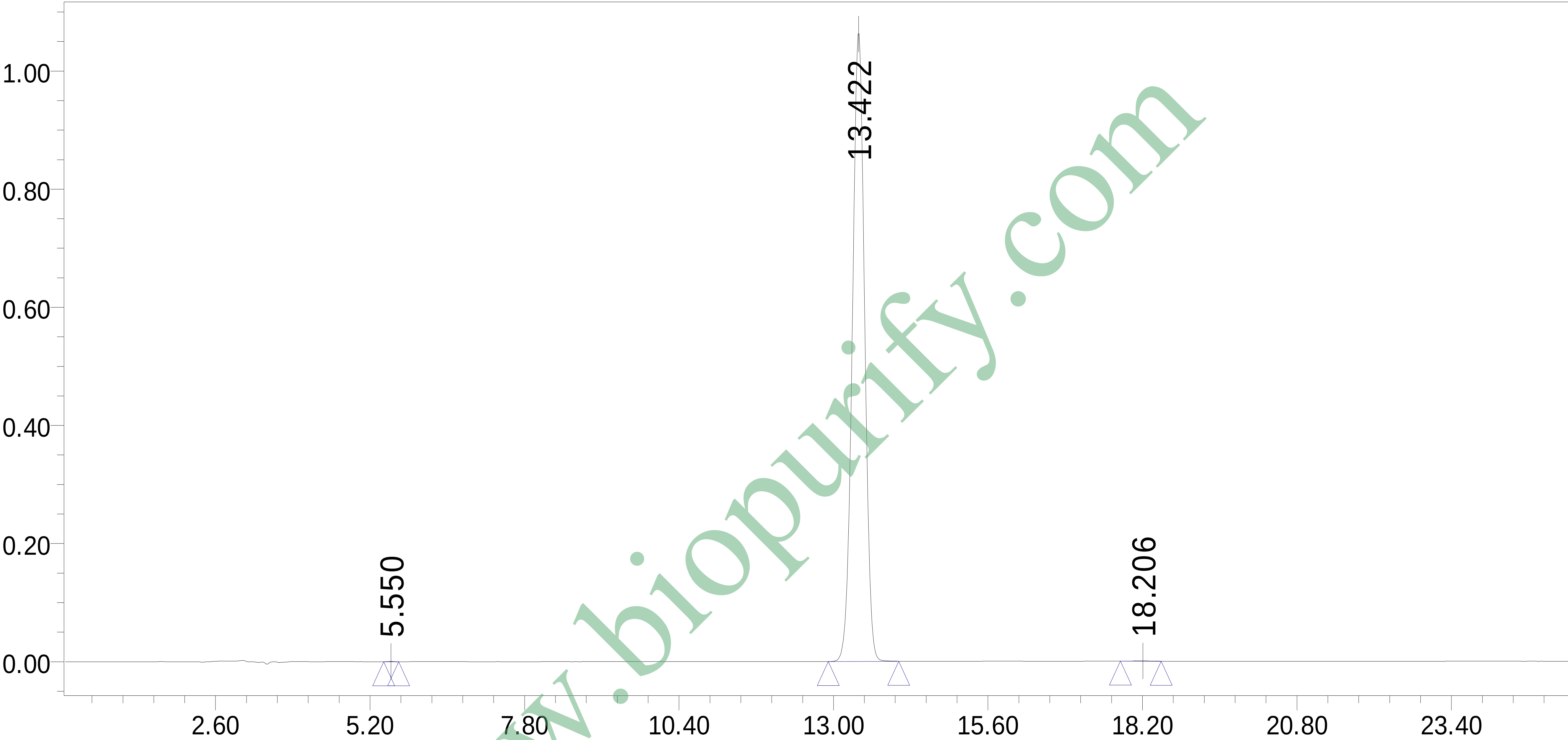
Auto-Scaled Chromatogram
