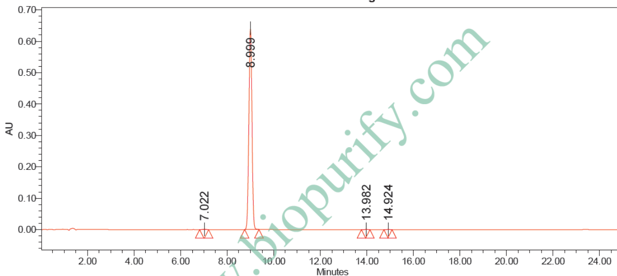
Auto-Scaled Chromatogram
