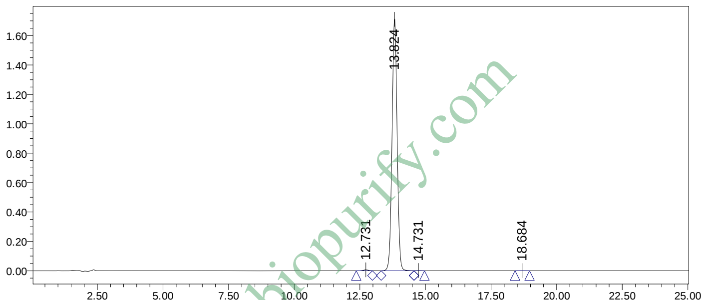
Auto-Scaled Chromatogram
