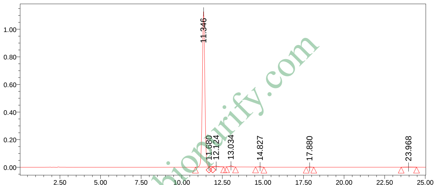
Auto-Scaled Chromatogram
