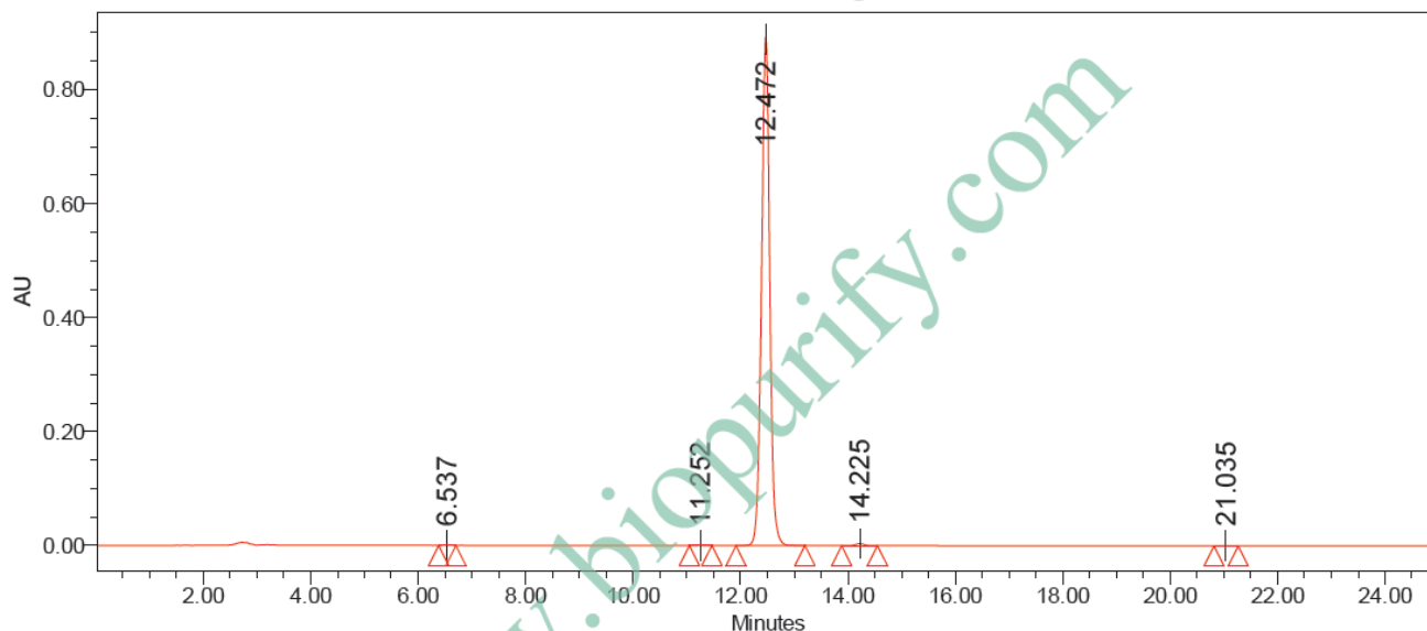
Auto-Scaled Chromatogram
