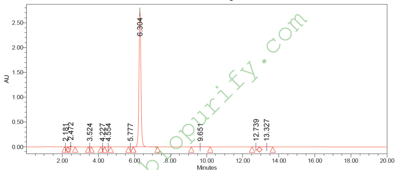
Auto-Scaled Chromatogram
