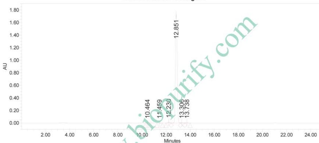
Auto-Scaled Chromatogram
