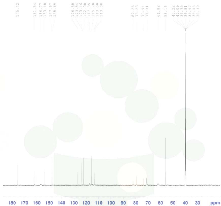
附 3b : ^{13}\text{C} -NMR(150M Hz , DMSO- \text{d}_6 )
