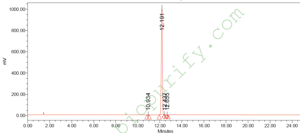
Auto-Scaled Chromatogram
